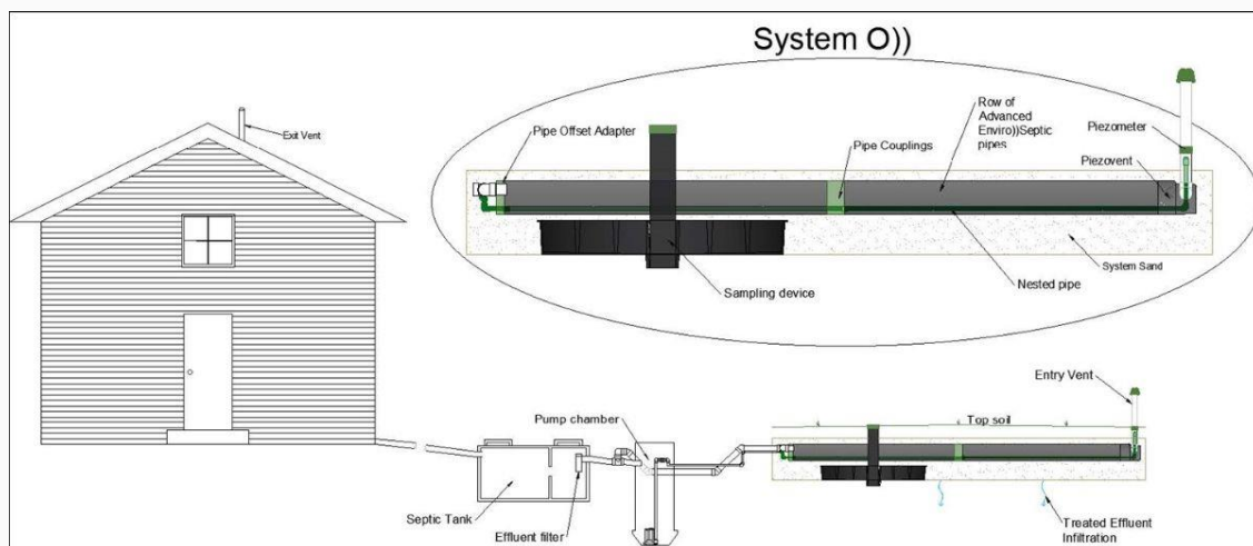
Figure 2: Nested Pipe Configuration, BMEC #23-06-408
