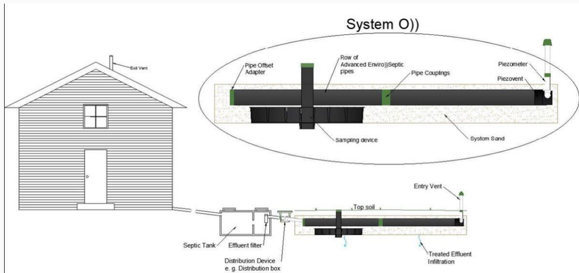
Figure 1: Standard Configuration, BMEC #23-05-407
