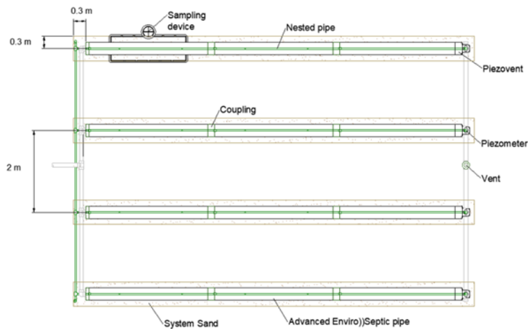
Top View – Nested Pipe Configuration
