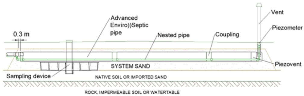
Side View – Nested Pipe Configuration
